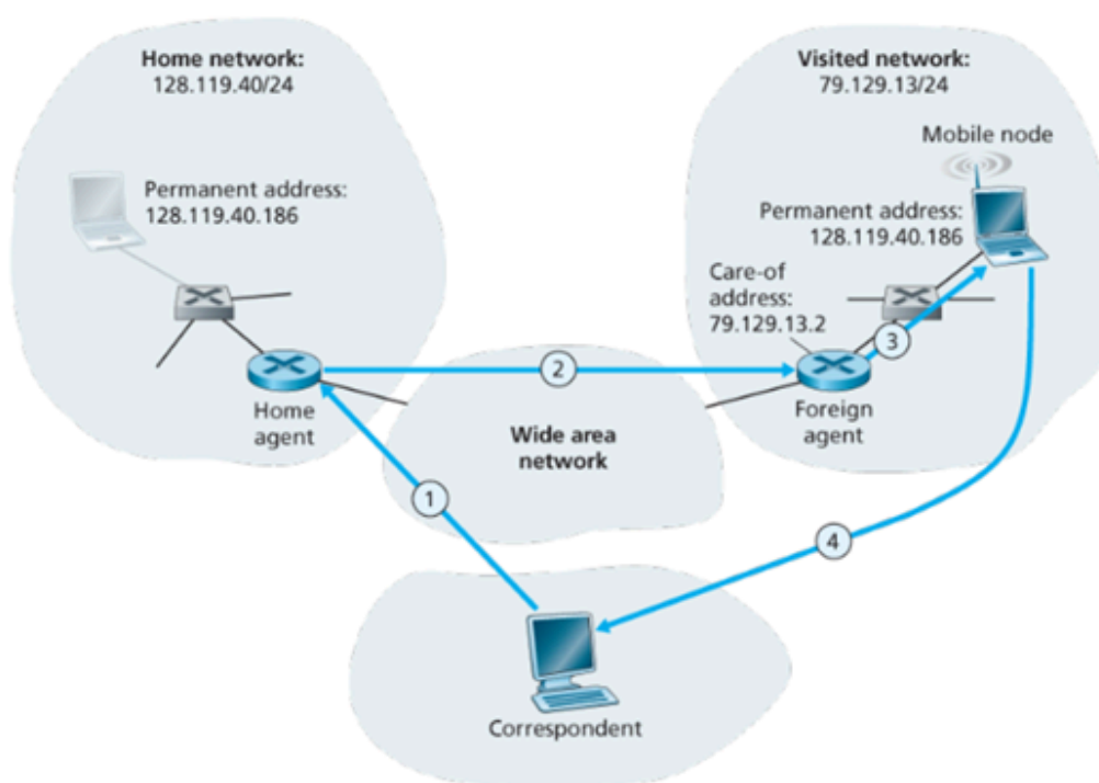
Figure 7.24 Indirect routing to a mobile node
